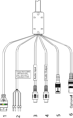
Figure2-2 Multi-head cable 2
