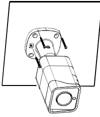
Figure 3-1 Installing camera
